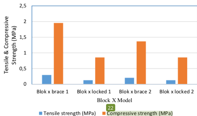
Figure 6. Graph of tensile strength and compressive strength of type x blocks
